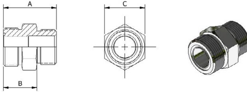
SAE Male To ORFS Male Adapter - DM60166
