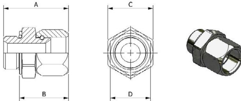
BSPP Male To JIC Female Swivel Adapter - DM80158
