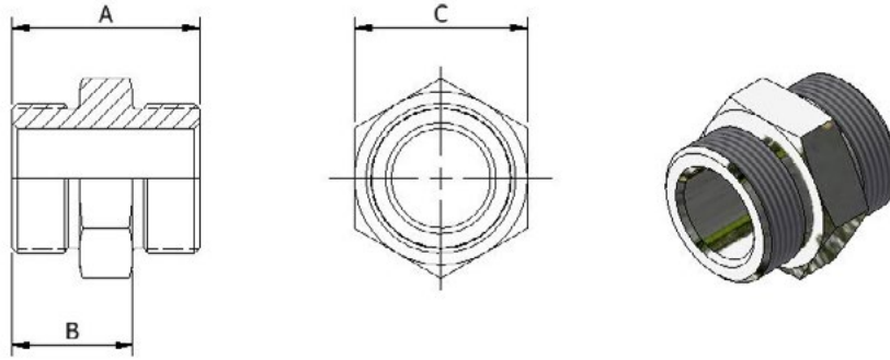
SAE Male To SAE Male Adapter - DM60157
