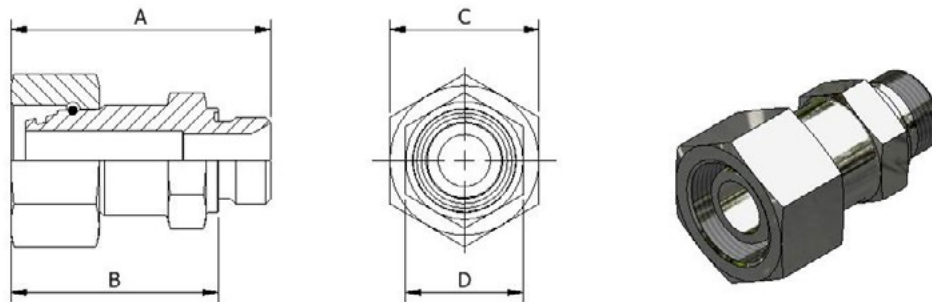
BSPP Male To DIN Female Swivel Adapter - DM80167
