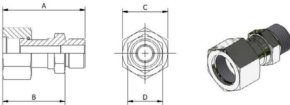
SAE Male To ORFS Female Swivel Adapter - DM60156
