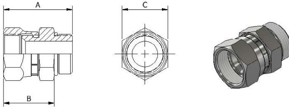
SAE Male To JIC Female Swivel Adapter - DM60155
