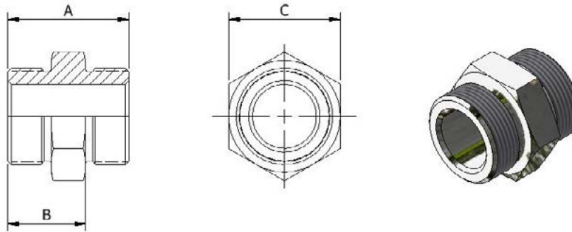
SAE Male To SAE Male Adapter - DM60157
