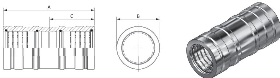
Coupling with Inner Stop, OD Tube - DM60002
