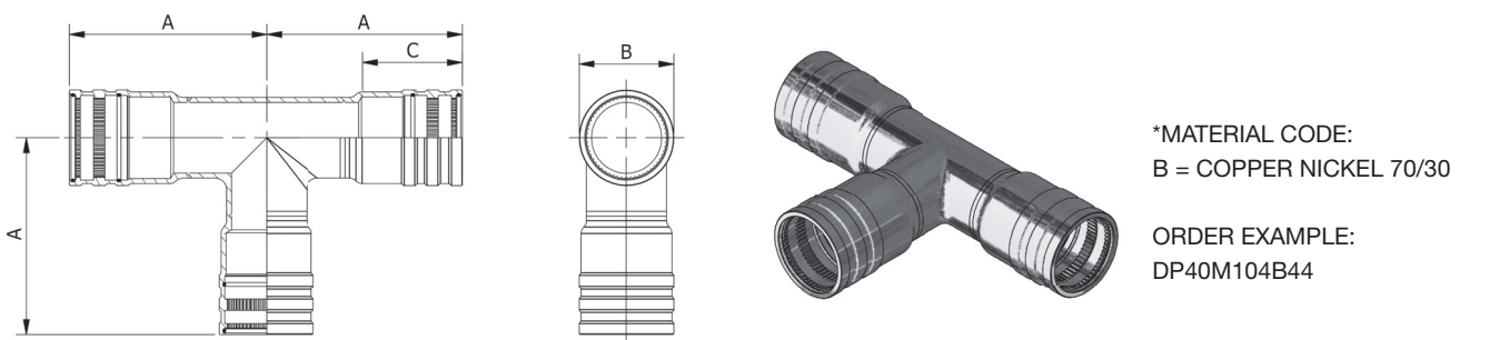
Low Pressure Reducing Tee - DP40M104
