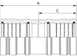
Coupling with Inner Stop, Metric, JIS - DM80002
