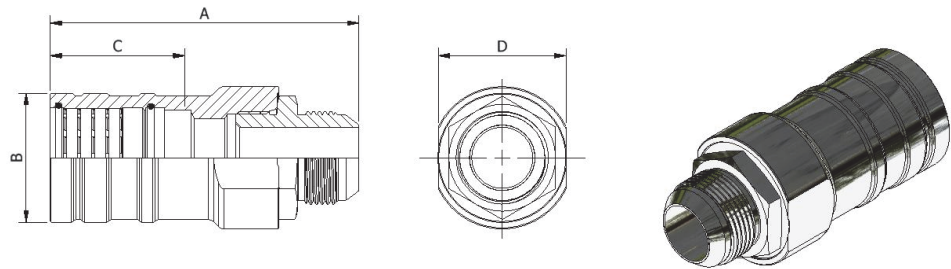
JIC 37° Male, OD Tube - A-DM60055 (Assembly - Comprises DM60087 & DM60164)
