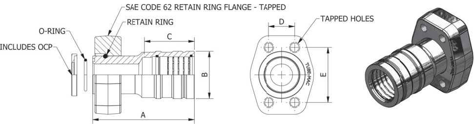
SAE Code 62 Tapped Flange, OD Tube - DM60096
