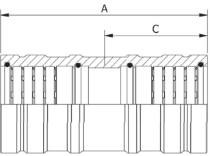
Coupling, Metric, JIS - DM8000
