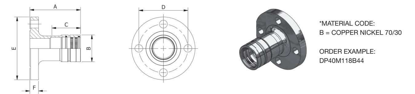
Flange – ANSI #150, Metric - DP40M018
